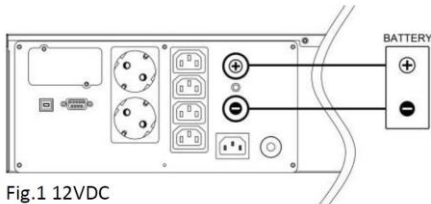
Fig.1 12VDC
