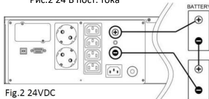
Fig.2 24VDC
