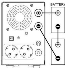
Fig.2 24VDC
