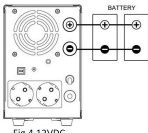
Fig.4 12VDC
