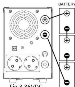
Fig.3 36VDC
