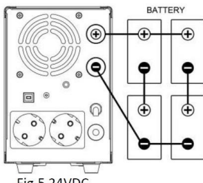
Fig.5 24VDC
