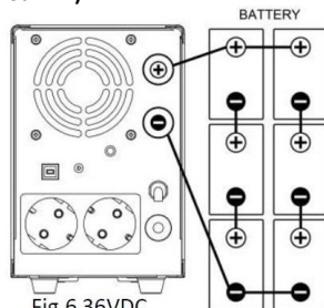
Fig.6 36VDC
