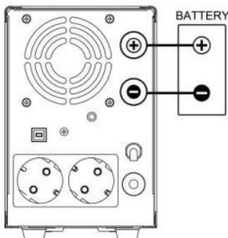
Fig.1 12VDC
