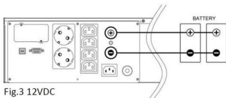
Fig.3 12VDC
