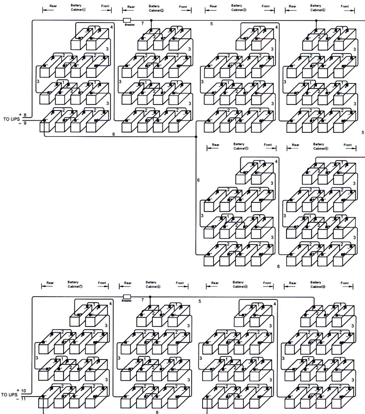
DGL100348B5Ⅳ(A), DGL100348B5 V (A), DGL100348B5Ⅵ(A), DGL100348B5Ⅶ(A) Wiring connection
